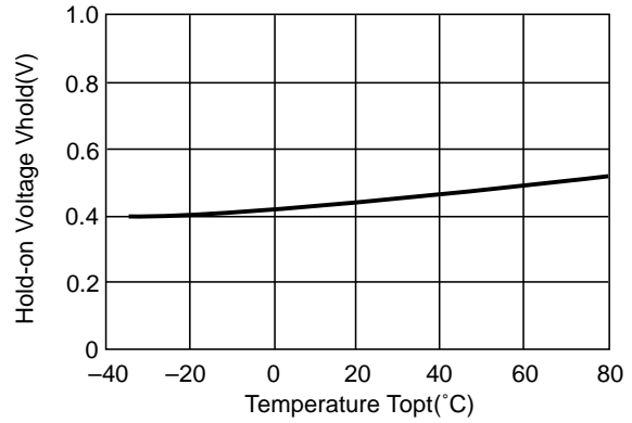
8) Hold-on Voltage vs. Temperature
